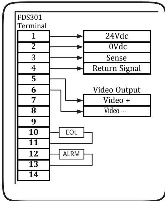
Figure 12: 4 Pair Termination
