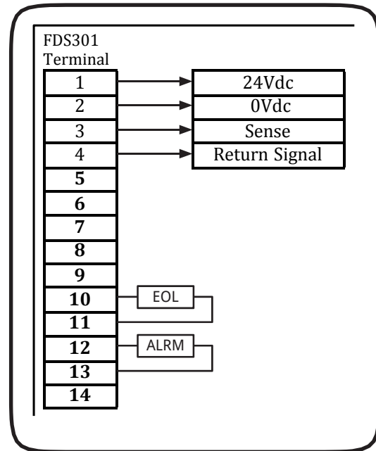
Figure 11: 2 Pair Termination
