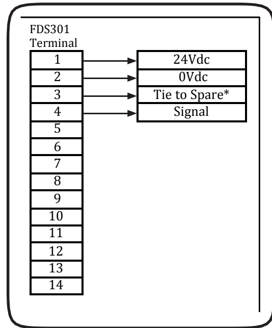
Figure 8: 4 Pair Termination
