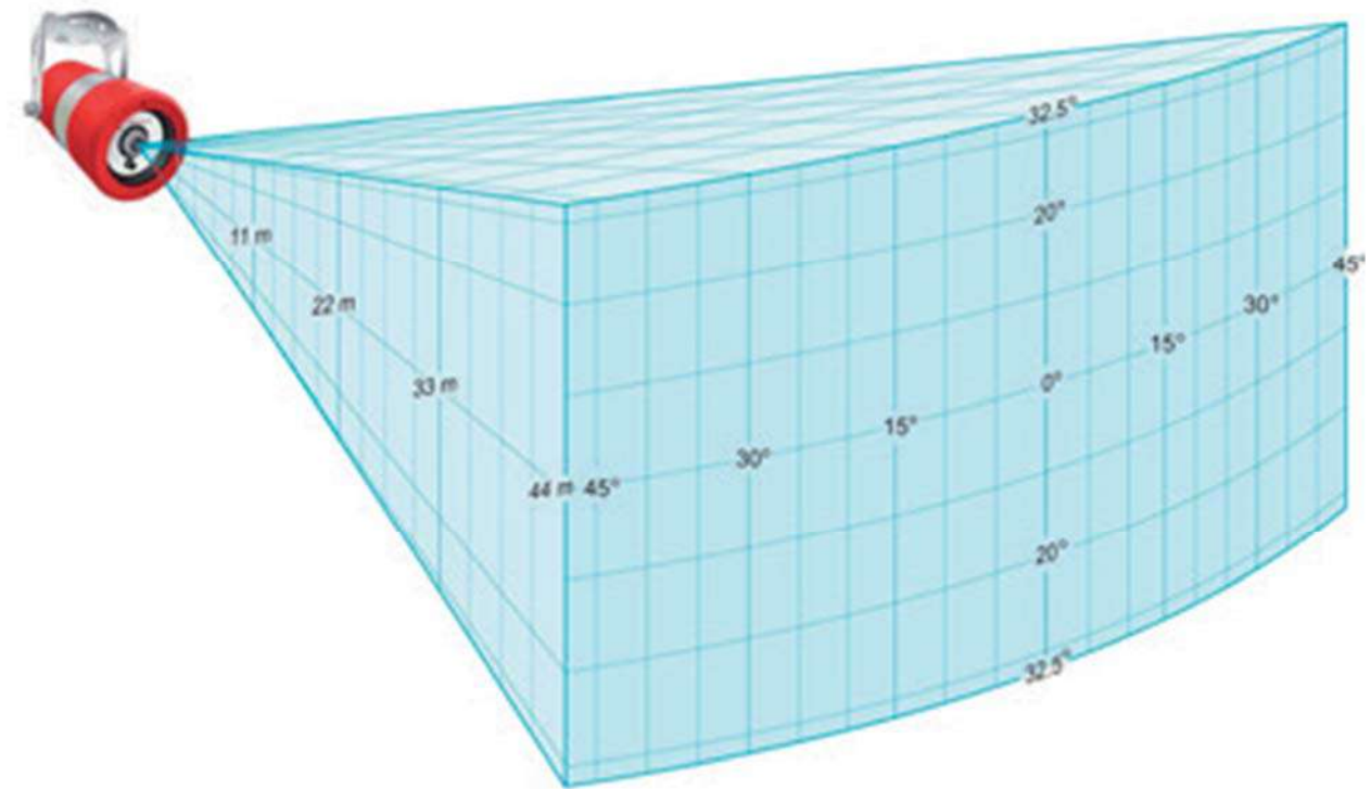
Figure 14: FDS301 Coverage & Field of View
