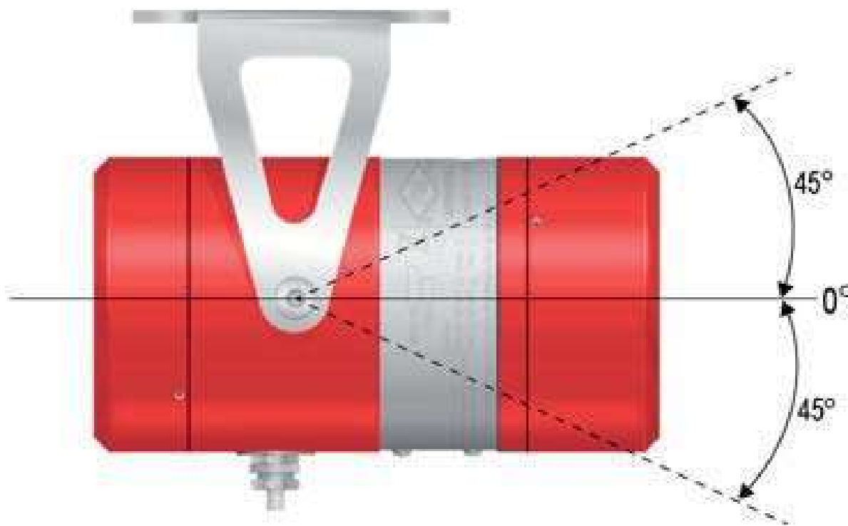
Figure 2: FDS301 Ceiling Mount
