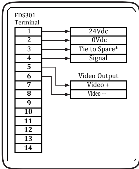
Figure 7: 3 Wire Termination
