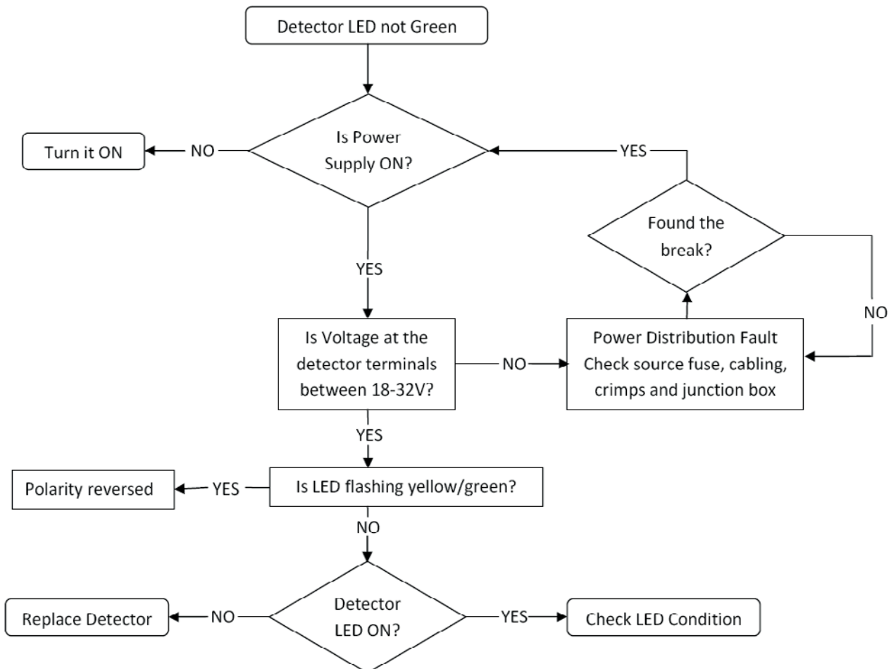
Figure 16: Power Supply Diagnostic Chart
