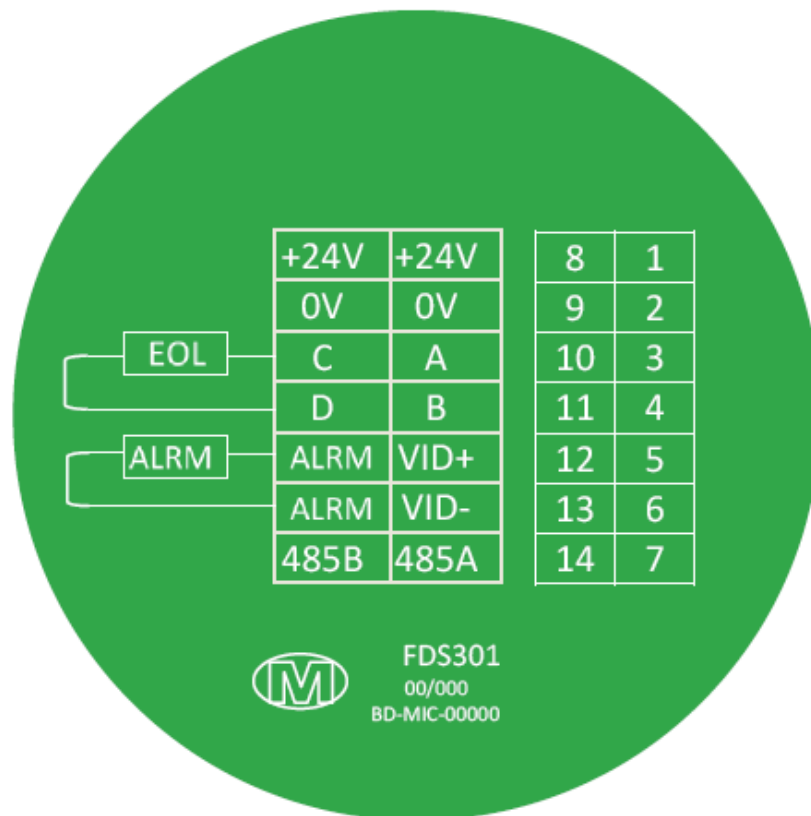
Figure 4: Terminal Schematic
