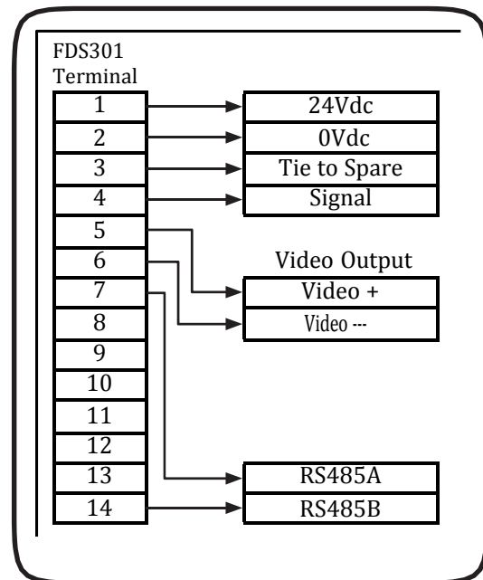
Figure 8: 4 Pair Termination
